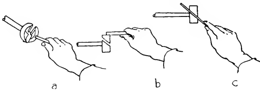
FIG. 107. SHARPENING FORSTNER BIT.
